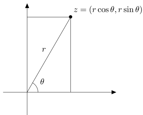
Figure 83: Complex number represented by radius and angle
