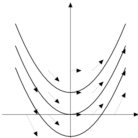
Figure 79: The integral curves of y'(x) = x .
