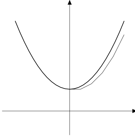
Figure 80: The Euler method to solve y'(x) = x with (x_0, y_0) = (0, 1) with \epsilon = 0.5 .
