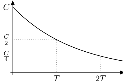
Figure 78: The exponential decay y(x) = Ce^{-ax} = C2^{-ax/\log 2} . The half-life is T = \log 2/a .
