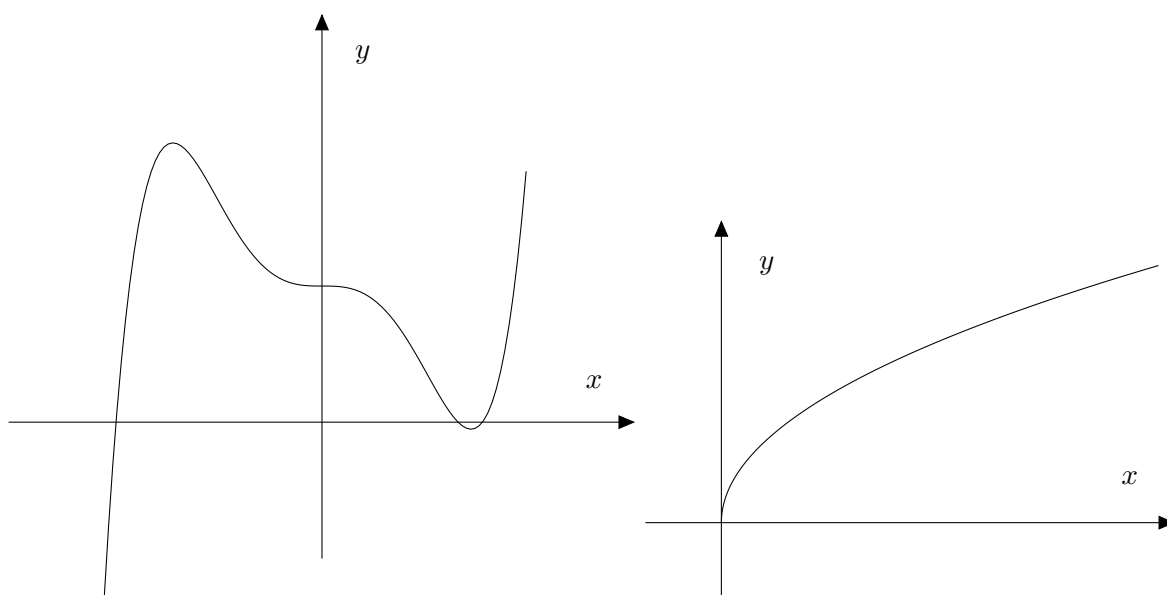
Figure 11: Left: the graph of y = x^5 - 2x^3 + 1 . Right: the graph of y = \sqrt{x} .
