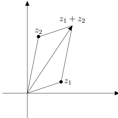
Figure 82: Sum of two complex numbers
