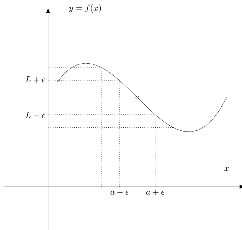
Figure 18: The limit \lim_{x \rightarrow a} f(x) .
