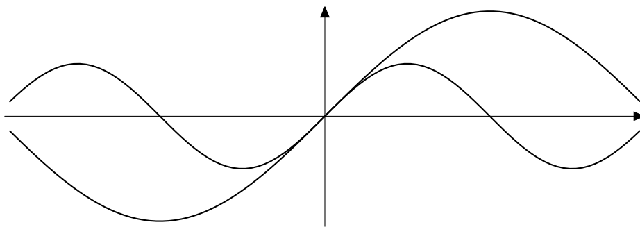
Figure 55: The graphs of \sin x and 2 \sin(x/2) .
