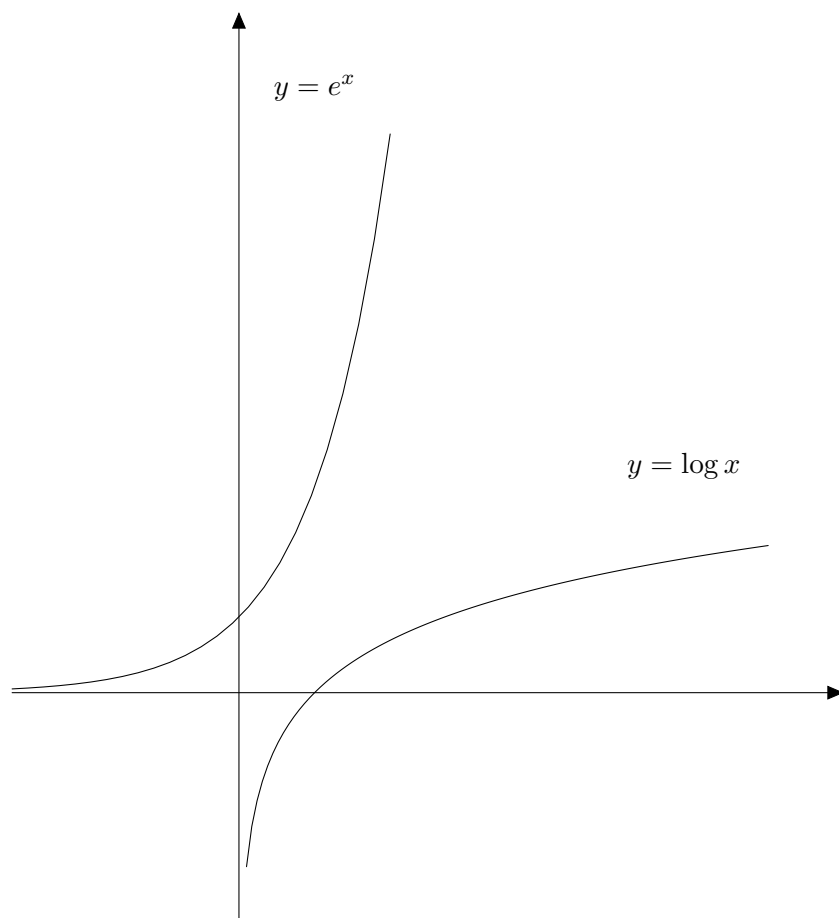
Figure 24: The logarithm and the exponential.
