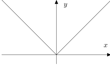
Figure 43: The graph of y = |x| , which has left and right derivatives, but they do not coincide.
