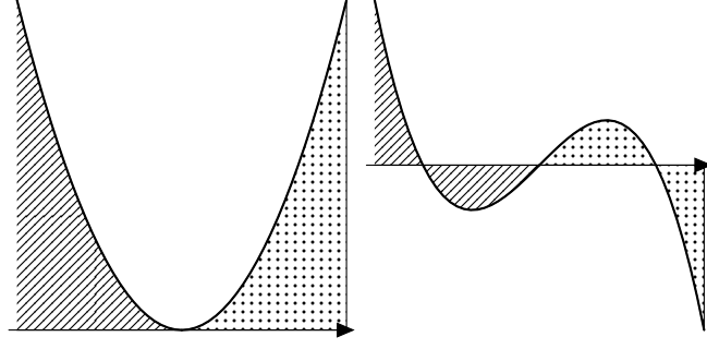
Figure 70: Integral of symmetric and antisymmetric functions.
