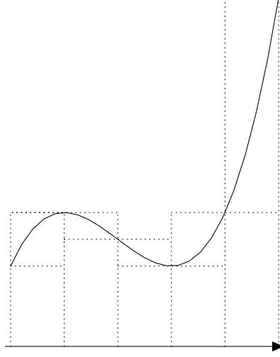
Figure 67: \overline{S}_I(f, P) and \underline{S}_I(f, P) for a given a partition P of I .
