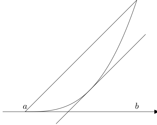
Figure 48: A function continuous in [a, b] and differentiable in (a, b) , must have a point where the derivative is equal to the mean slope.
