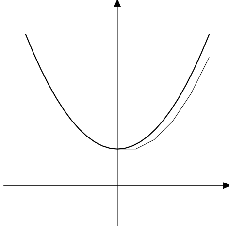
Figure 79: The Euler method to solve y' = x with (x_0, y_0) = (0, 1) with \epsilon = 0.5 .
