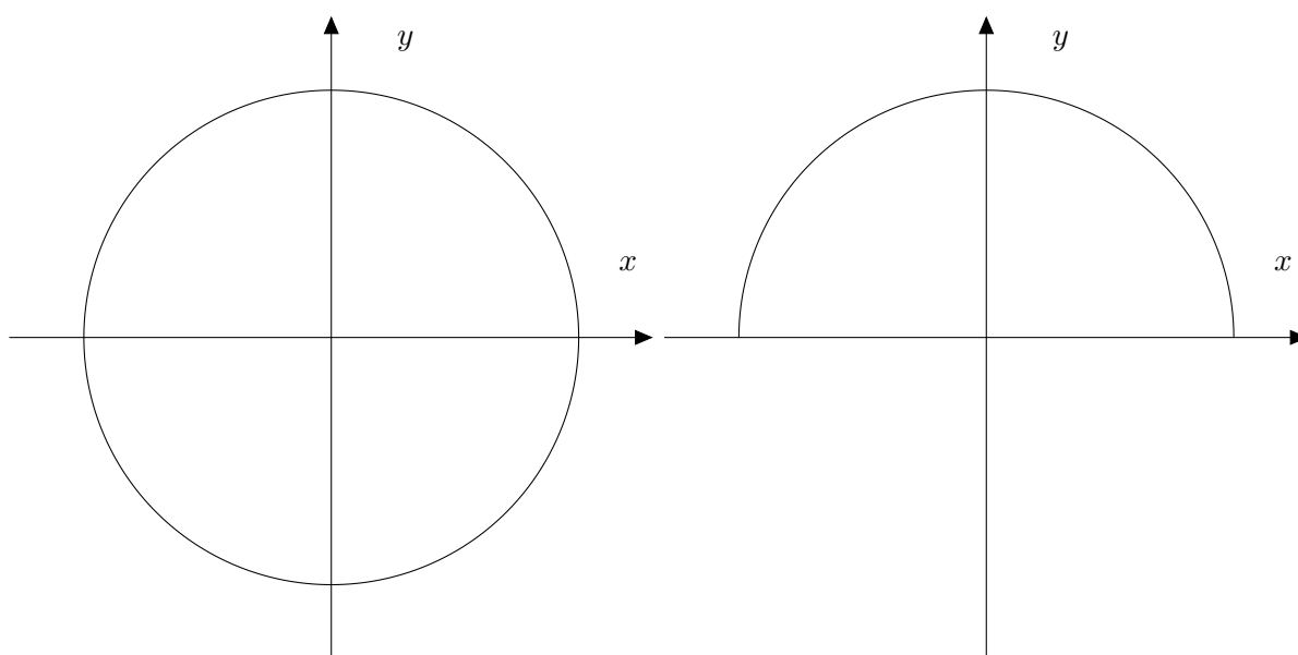
Figure 11: Left: the graph of x^2 + y^2 = 1 , not a function of x . Right: the graph of y = \sqrt{1 - x^2} .
