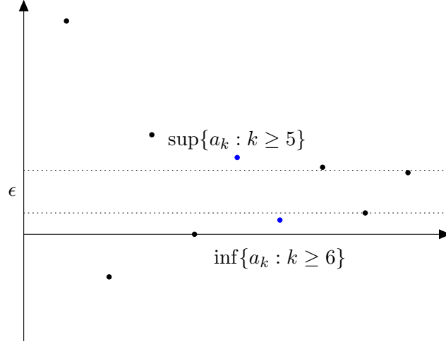
Figure 22: A Cauchy sequence.
