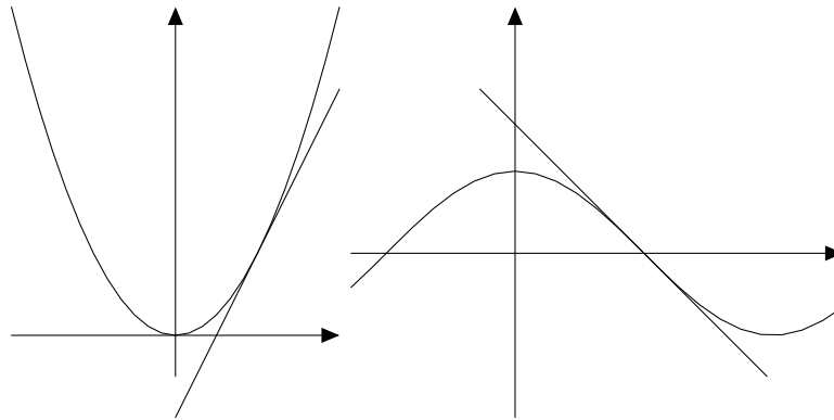
Figure 45: The tangent lines to the graphs of x^2, \cos x . Their equations are y = 2(x - 1) + 1, y = -(x - \frac{\pi}{2}) , respectively.
