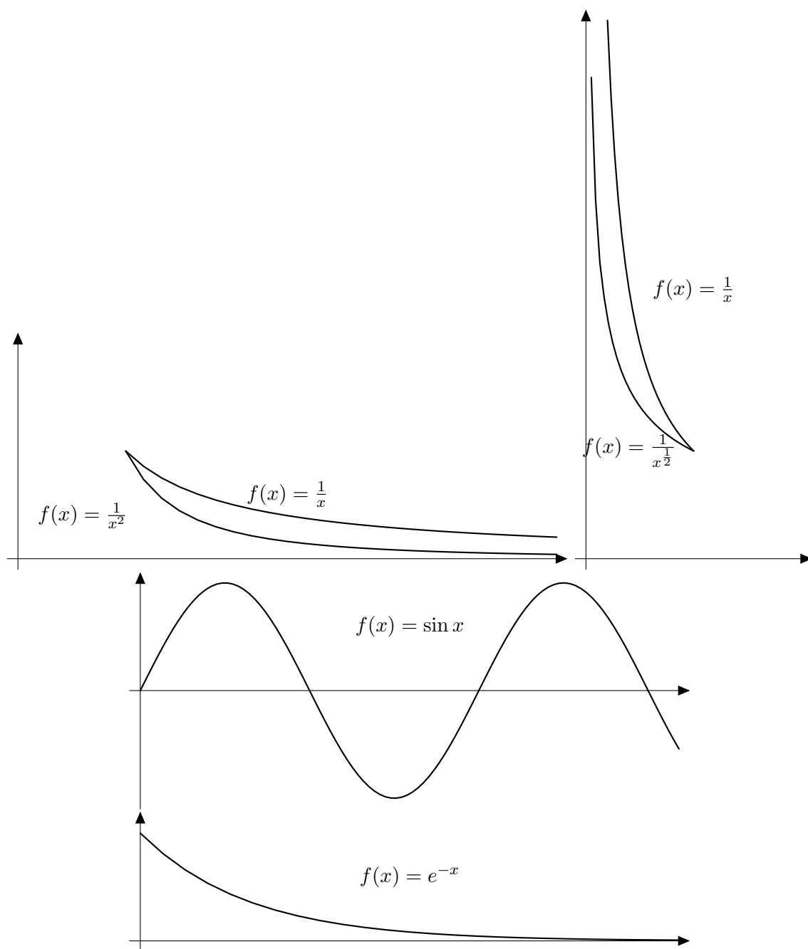
Figure 71: Convergent and non convergent improper integrals.
