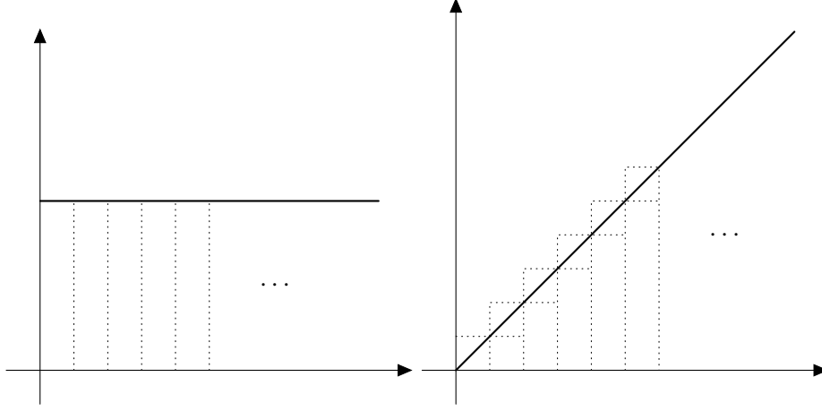
Figure 68: The upper and lower sum for f(x) = a (constant) and f(x) = x .
