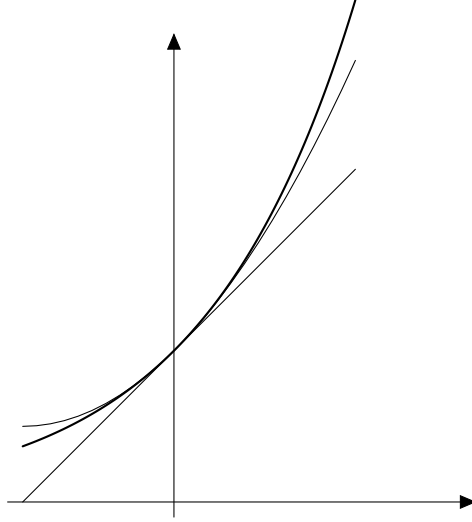
Figure 63: The second order Taylor formula. We approximate a general function by a second order polynomial.
