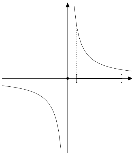
Figure 36: A continuous function on a bounded closed interval is bounded. If either of these conditions are violated, then function can be unbounded.
