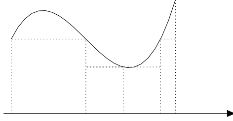
Figure 65: Approximating the area surrounded by f(x) by rectangles.
