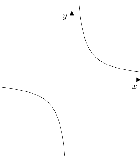
Figure 13: The graphs of y = \frac{1}{x} on (-\infty, 0) \cup (0, \infty) .
