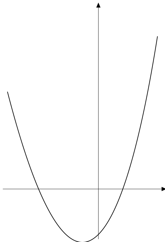
Figure 59: The graph of h(x) = e^x + x^2 - 2 . It crosses the x -axis twice and only twice.
