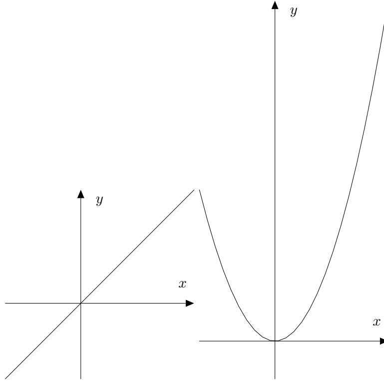
Figure 9: Left: the graph of y = x . Right: the graph of y = x^2 .
