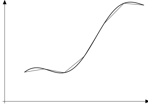
Figure 76: The length and segments.
