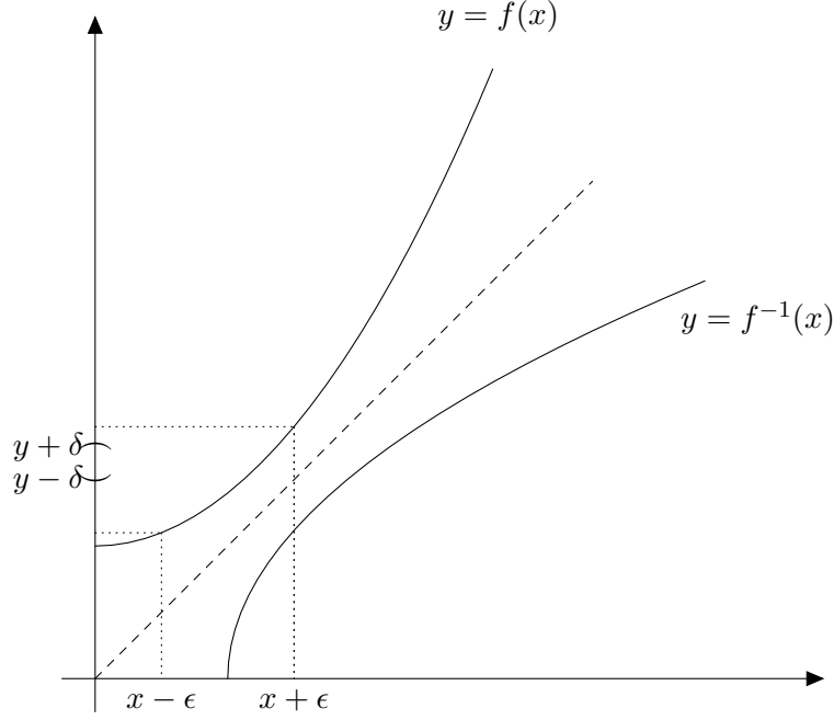
Figure 21: The continuity of the inverse function. For a given \epsilon , we can take \delta .
