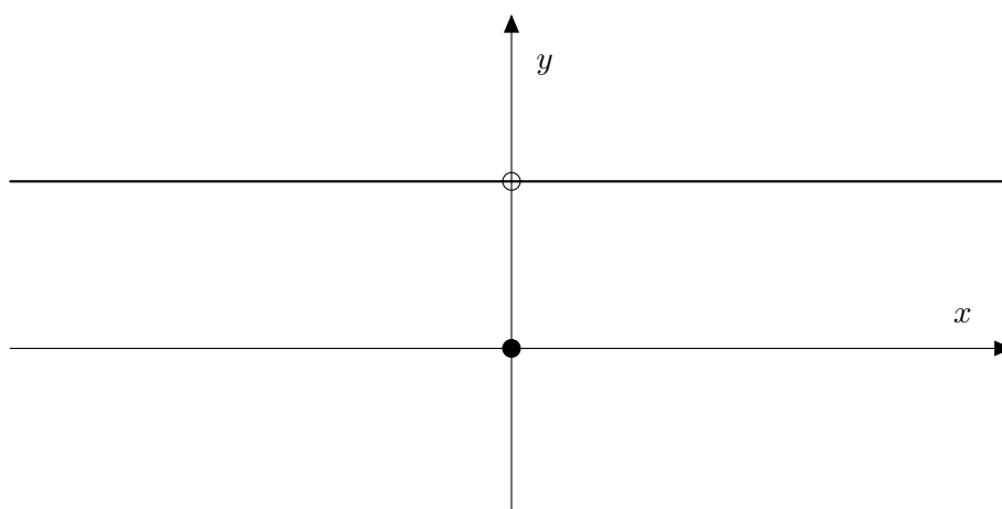
Figure 19: The graph of y = \begin{cases} 1 & \text{if } x \neq 0 \\ 0 & \text{if } x = 0 \end{cases} .
