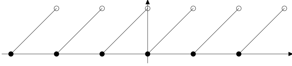
Figure 38: The graph of the function y = x - [x] , the decimal part of x . This is bounded, but has no maximum. The minimum is 0 at x \in \mathbb{Z} .
