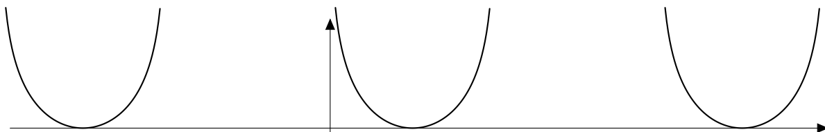
Figure 58: The graph of f(x) = \log(\frac{1}{\sin x}) .
