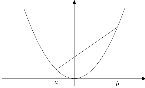
Figure 51: A convex function. The graph is below the segment between any pair of points (a, f(a)), (b, f(b)) .
