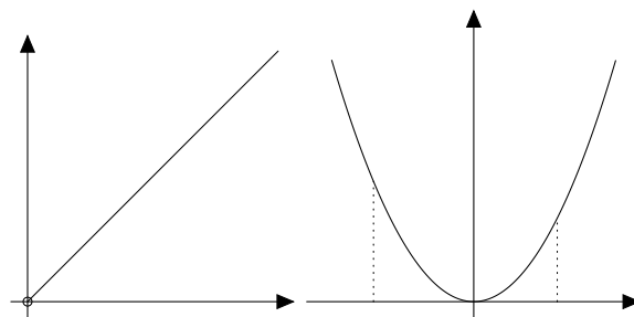
Figure 37: Left: y = x on x > 0 . There are no minimum or maximum. Right y = x^2 on \mathbb{R} . The minimum is 0 at x = 0 , but there is not maximum. When restricted to [a, b] , either a^2 or b^2 is the maximum.
