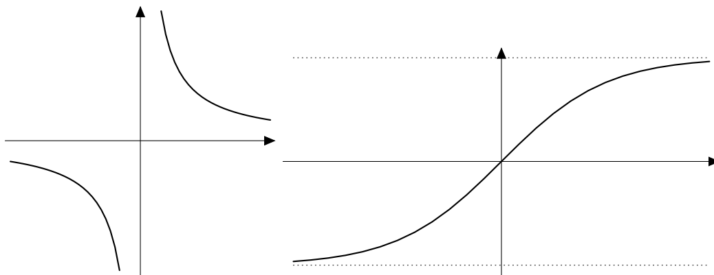
Figure 52: The asymptotes for \frac{1}{x} and \tanh x .
