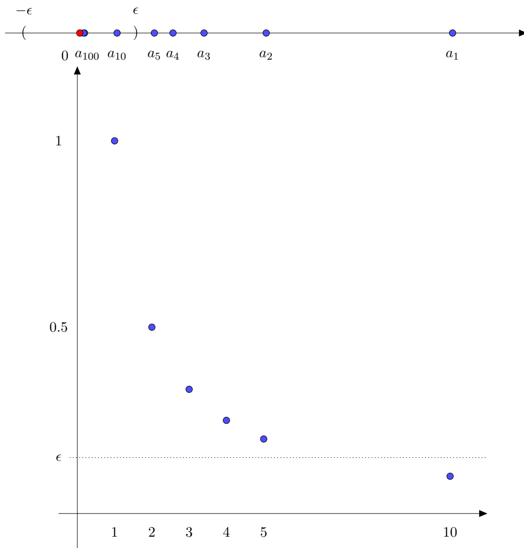
Figure 15: Up: the sequence a_n = \frac{1}{n} plotted on the line. Bottom: the sequence a_n = \frac{1}{n} as a function on \mathbb{N} .
