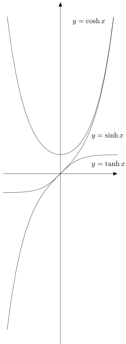
Figure 27: The hyperbolic functions.
