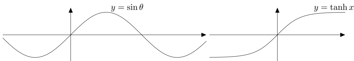
Figure 40: Functions defined on \mathbb{R} but uniformly continuous.
