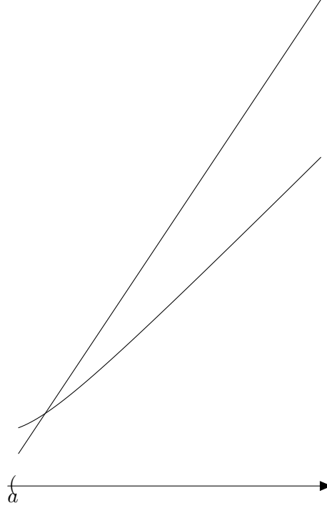
Figure 61: Theorem of de l'Hôpital. The limit \lim_{x \rightarrow \infty} \frac{f(x)}{g(x)} is determined by \lim_{x \rightarrow \infty} \frac{f'(x)}{g'(x)} .
