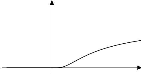
Figure 64: The graph of a function whose Taylor series converges but not to itself.
