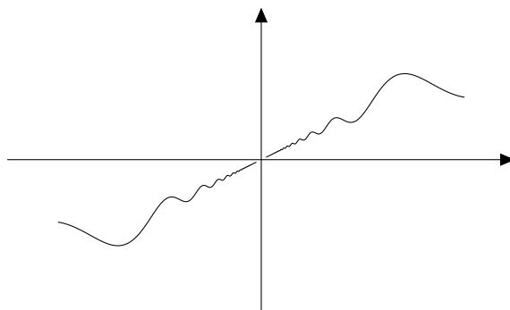
Figure 50: A function f such that f'(0) > 0 but is not monotonically increasing in any interval containing x = 0 .
