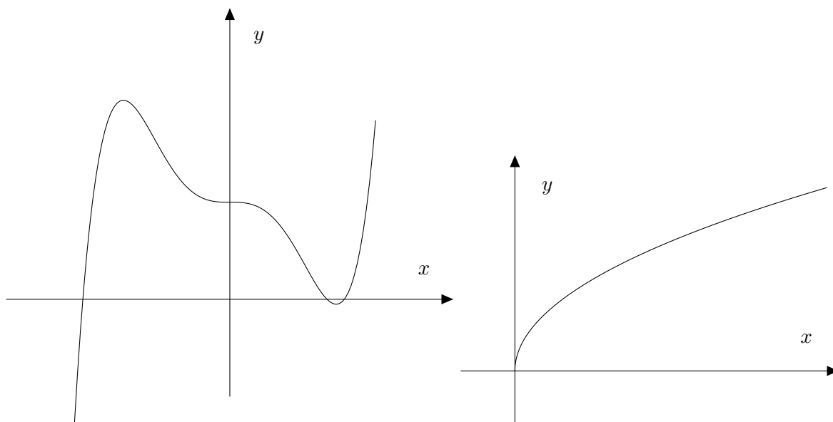
Figure 10: Left: the graph of y = x^5 - 2x^3 + 1 . Right: the graph of y = \sqrt{x} .
