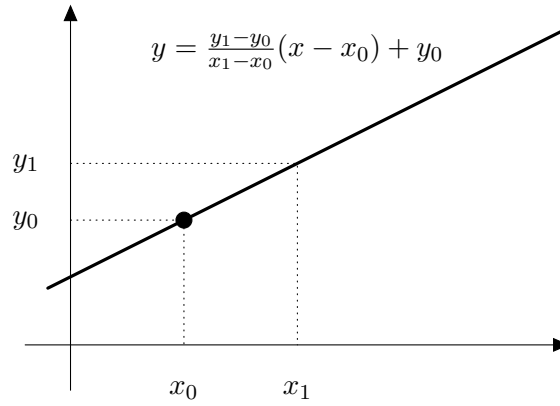
Figure 44: The slope of the straight line is \frac{y_1 - y_0}{x_1 - x_0} .
