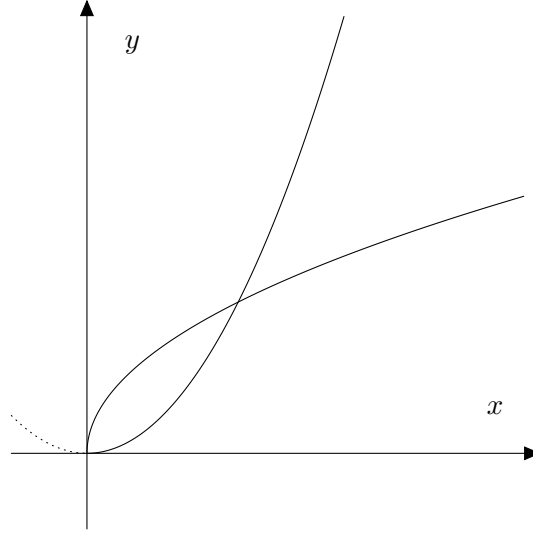
Figure 14: The graphs of y = \sqrt{x} and y = x^2 on [0, \infty) .
