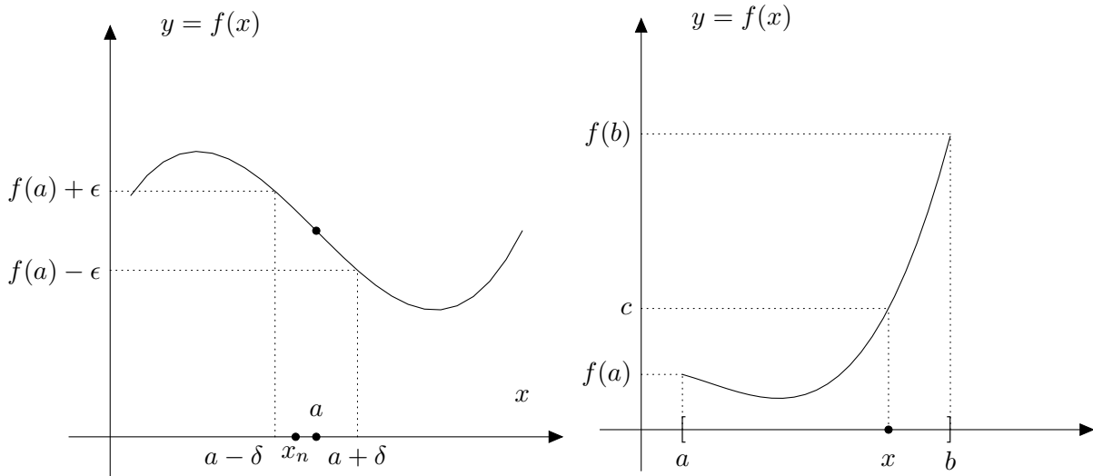
Figure 20: Left: continuity of f and a sequence x_n \rightarrow a . Right: the intermediate value c is taken at x .
