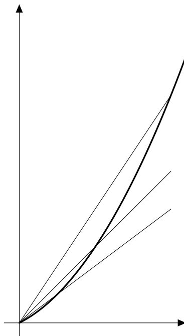
Figure 41: The slope at a point as the limit of the slopes of secant lines.
