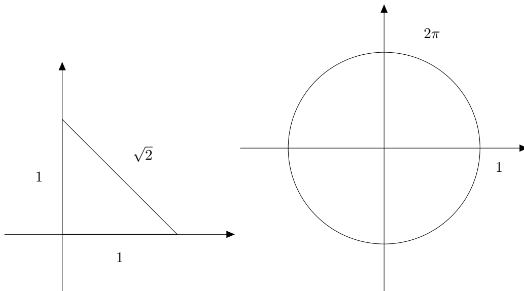
Figure 4: Left: the right triangle with equal sides 1. By the Pythagoras' theorem, the longest side is \sqrt{1^2 + 1^2} = \sqrt{2} . Right: the unit circle with radius 1 (diameter 2). The length of the circle (the circumference) is 2\pi .
