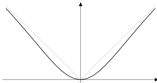
Figure 53: The oblique asymptotes for x \tanh x .
