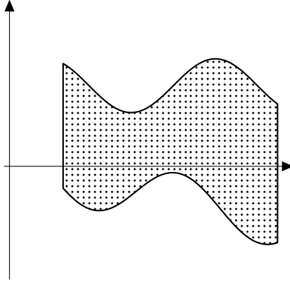
Figure 74: The area of the region between two functions.
