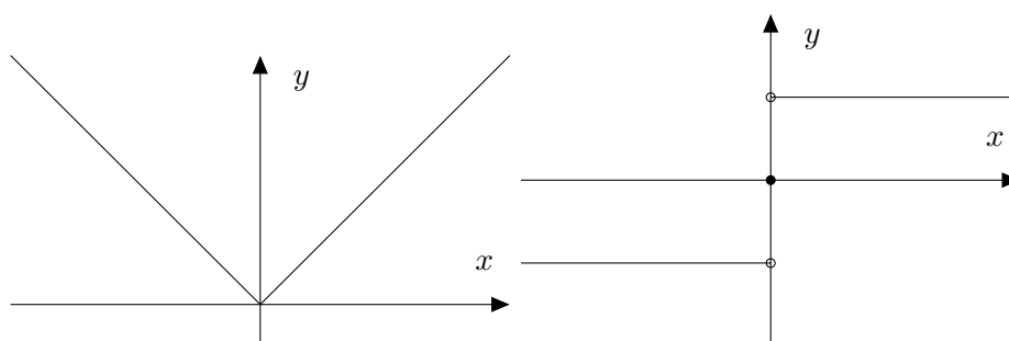
Figure 12: Left: the graph of y = |x| . Right: the graph of y = \text{sign } x , with a “jump” at x = 0 .
