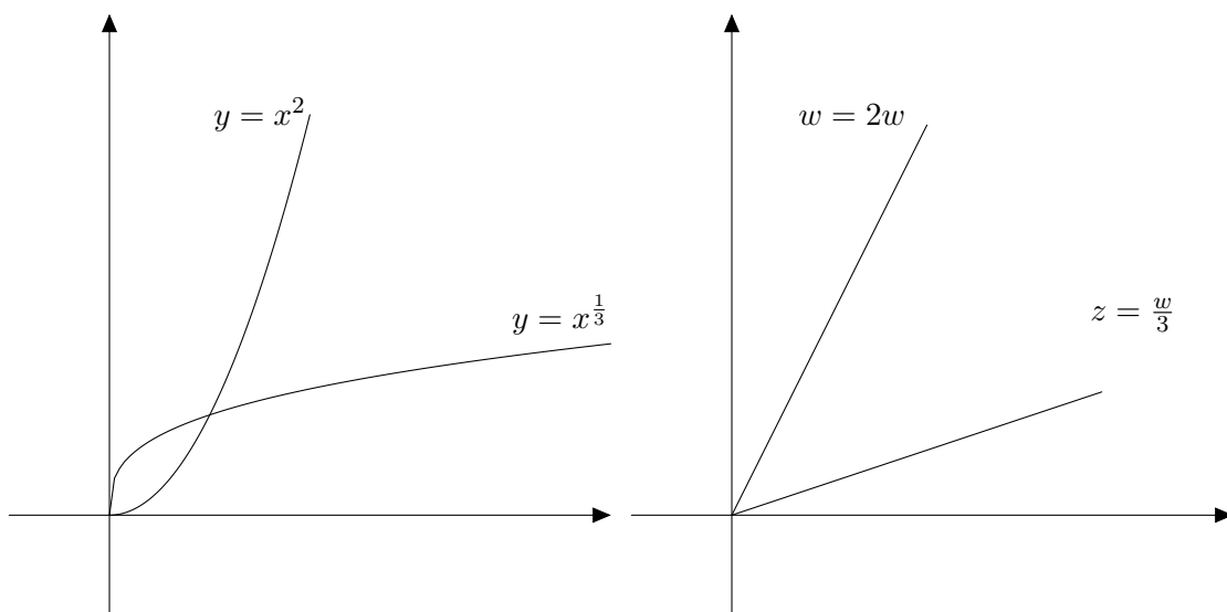
Figure 26: The log-log plot of the relation y = x^p .
