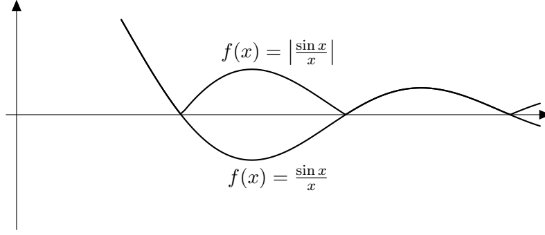
Figure 73: f(x) = \frac{\sin x}{x} and f(x) = \left| \frac{\sin x}{x} \right| . The improper integral of the former in [1, \infty) is convergent, while the latter is not.
