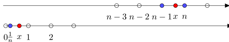
Figure 6: Any x \in \mathbb{R} falls between n - 1 and n (including equality) for some n \in \mathbb{N} . For any x > 0 , there is n \in \mathbb{N} such that \frac{1}{n} < x .
