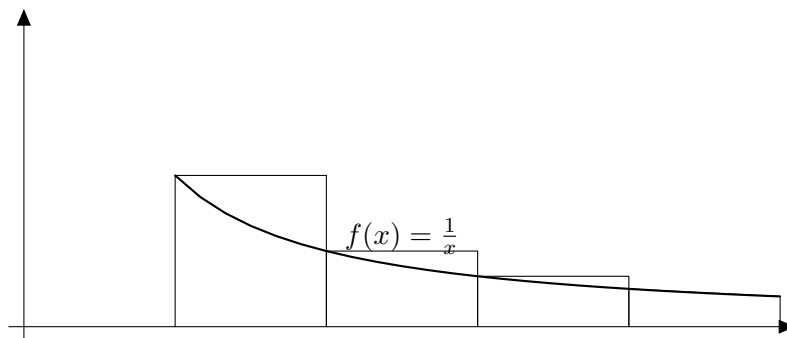
Figure 72: A graphical proof that \sum_{n=1}^N \frac{1}{n} diverges as N \rightarrow \infty .
