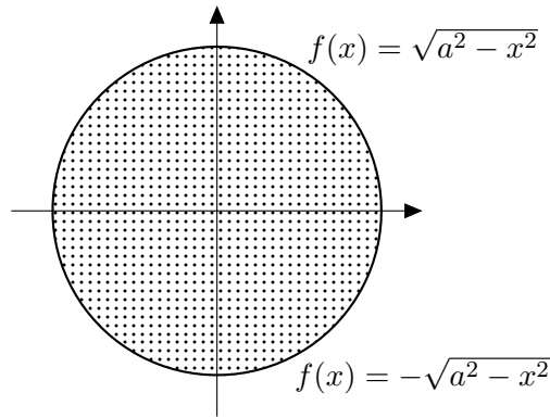
Figure 75: The area of a disk.
