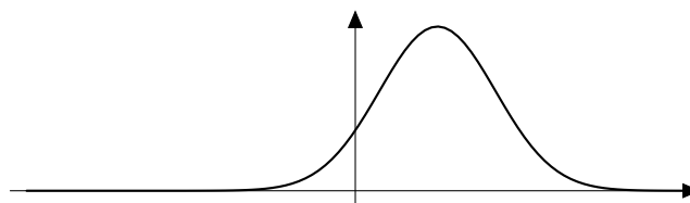
Figure 57: The graph of f(x) = e^{-(2x-1)^2} .
