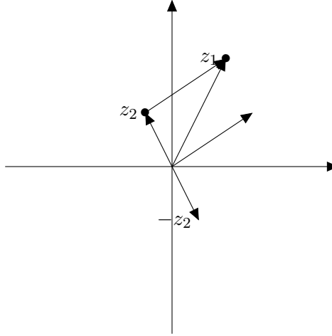
Figure 83: The distance of two complex numbers
