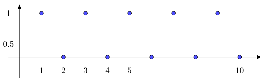
Figure 16: The sequence a_n = \frac{1}{2}(1 - (-1)^n) as a function on \mathbb{N} .
