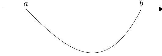
Figure 47: A non constant function, continuous in [a, b] and differentiable in (a, b) , must have a stationary point.
