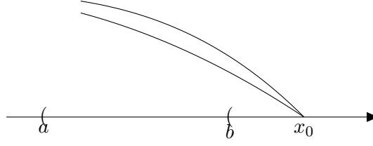
Figure 60: Theorem of de l'Hôpital. The limit \lim_{x \rightarrow x_0^-} \frac{f(x)}{g(x)} is determined by \lim_{x \rightarrow x_0} \frac{f'(x)}{g'(x)} .
