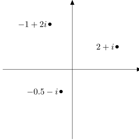
Figure 80: Various complex numbers on the plane
