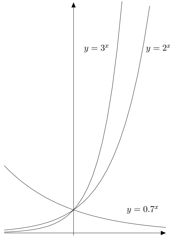
Figure 23: The exponential functions.
