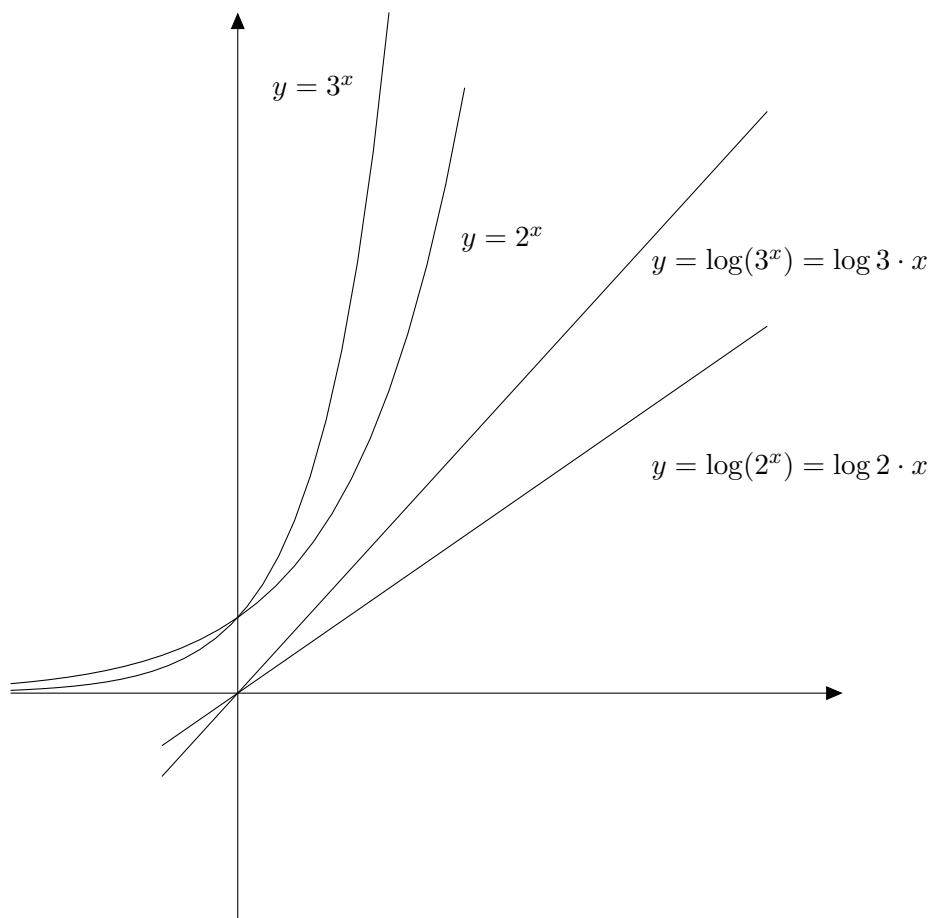
Figure 25: The exponential functions composed with the logarithm.
