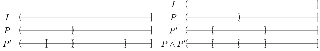
Figure 66: Left: a partition P of an interval I and a refinement P' \succ P . Right: two partitions P, P' of I and P \wedge P' .
