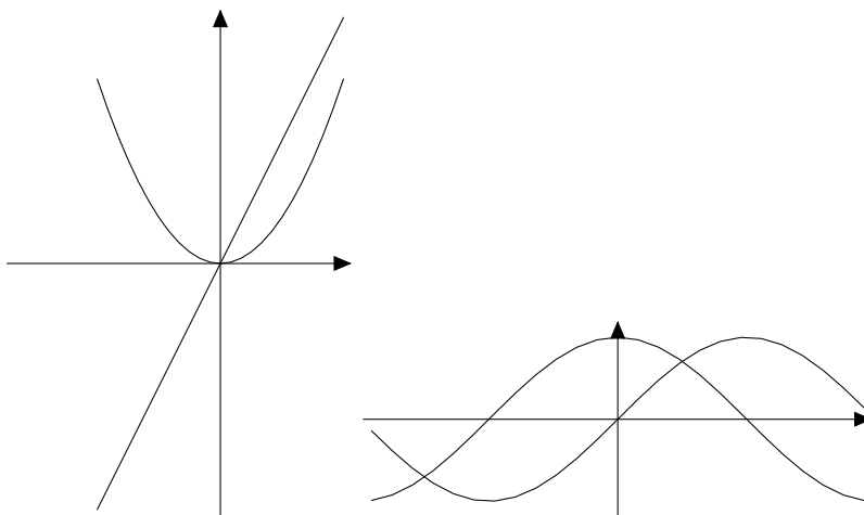
Figure 49: A function and its derivative. When the derivative is positive (negative) in an interval, the function is increasing (decreasing).
