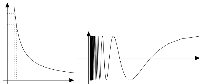
Figure 39: Functions continuous but not uniformly continuous.
