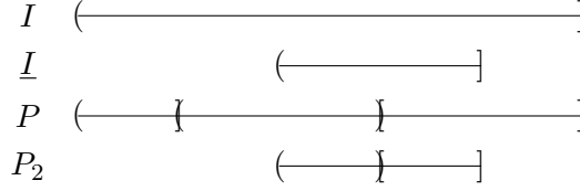
Figure 69: The partition P_2 of a subinterval \underline{I} of I obtained from a partition P of I .
