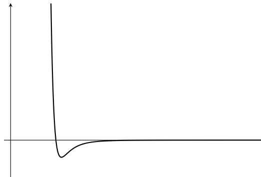
Figure 1.1: a Lennard-Jones potential
