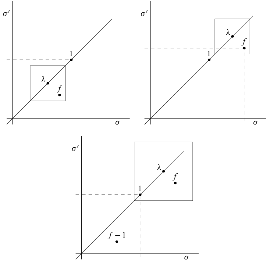
Figure 1. Top left: Since f is in the box of \lambda , it is in the box of 1. Top right: Since f is in the box of \lambda , 1 is in the box of f . Bottom: Since f is in the box of \lambda , f-1 is in the box of 1.
